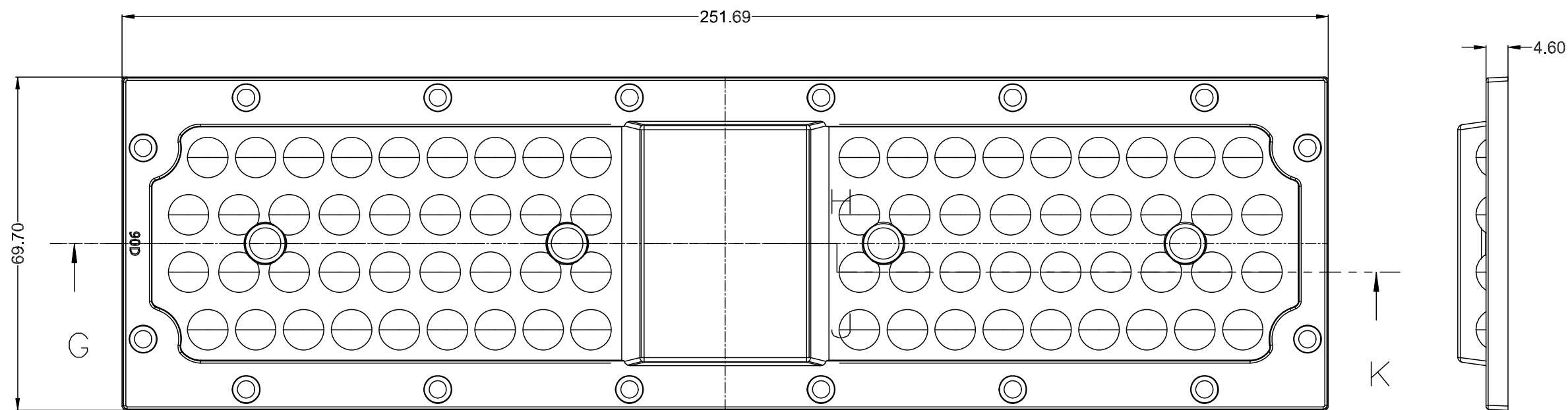
SECTION G-H-J-K
