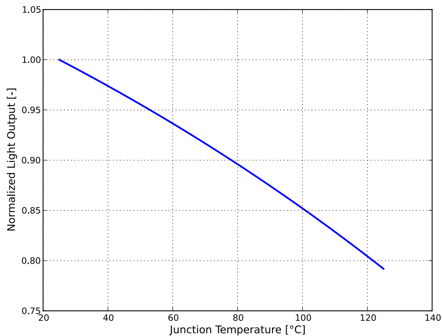
Figure 2. Typical normalized light output vs. junction temperature for all LUXEON 5050 at test current
