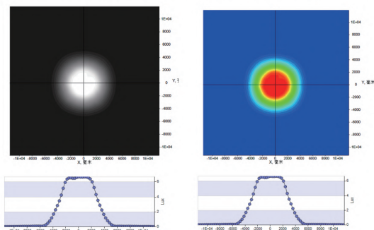
Total—Irradiance map for incident flux Black & Color (1m)
